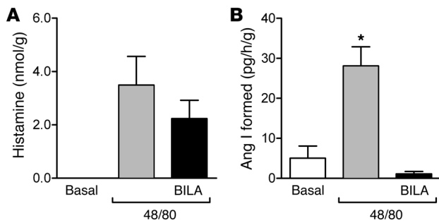
Figure 1 Coronary overflow of active renin (i.e., Ang I formed) and histamine from Langendorff-perfused guinea pig hearts challenged with the mast cell–degranulating compound 48/80 (300 µg) either in the absence or presence of the renin inhibitor BILA2157 (BILA; 100 nM). Bars indicate means ± SEM of overflow collected over 6 minutes either before (basal) or immediately following the administration of 48/80. (A) n = 7, 4, and 3, respectively; (B) n = 6, 3, and 3, respectively. *Significantly different from both basal and BILA2157-treated hearts. P < 0.05 by 1-way ANOVA with Dunnett’s procedure. Neither basal nor BILA2157-treated hearts were significantly different from 0 (1-sample Student’s t test).
